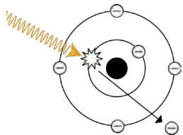
Photoelectric Effect
