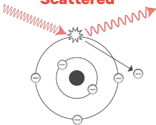
Compton Effect
